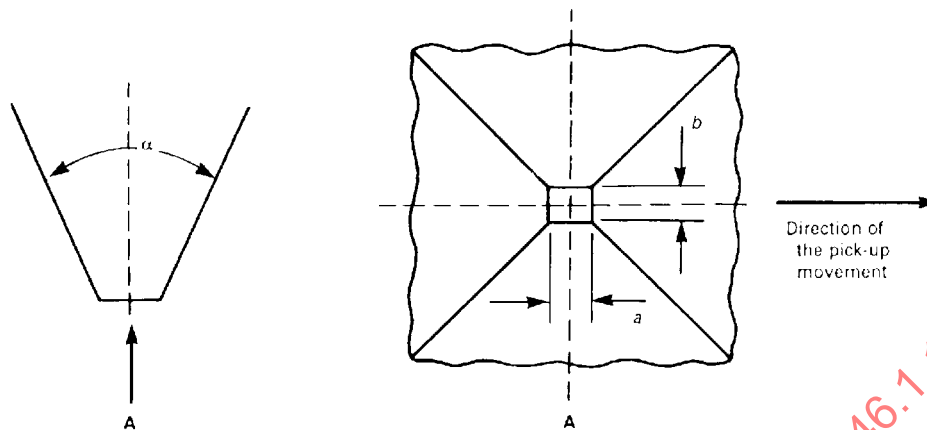
FIG. 3-3 TRUNCATED PYRAMID TIP
