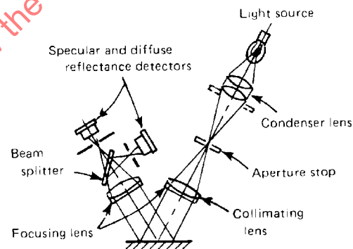
FIG. C2 REFLECTANCE MEASUREMENT
