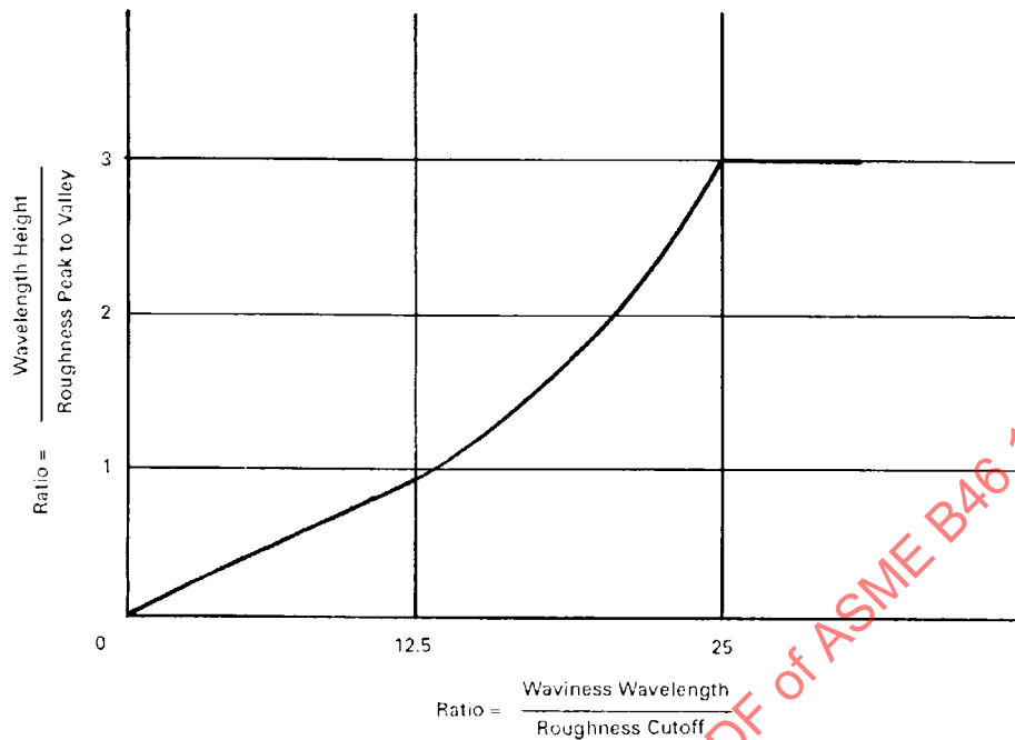
FIG. 11-3 ALLOWABLE WAVINESS
