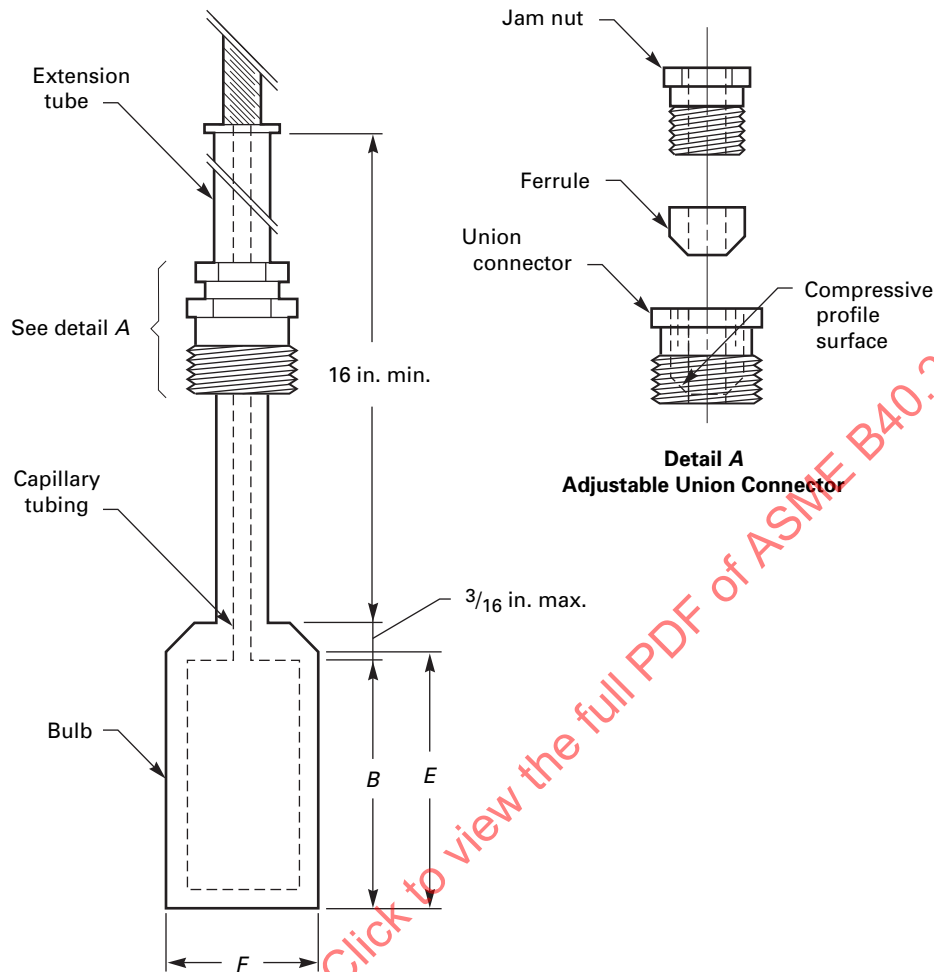
Fig. A-1 Class C Sensor Configuration
