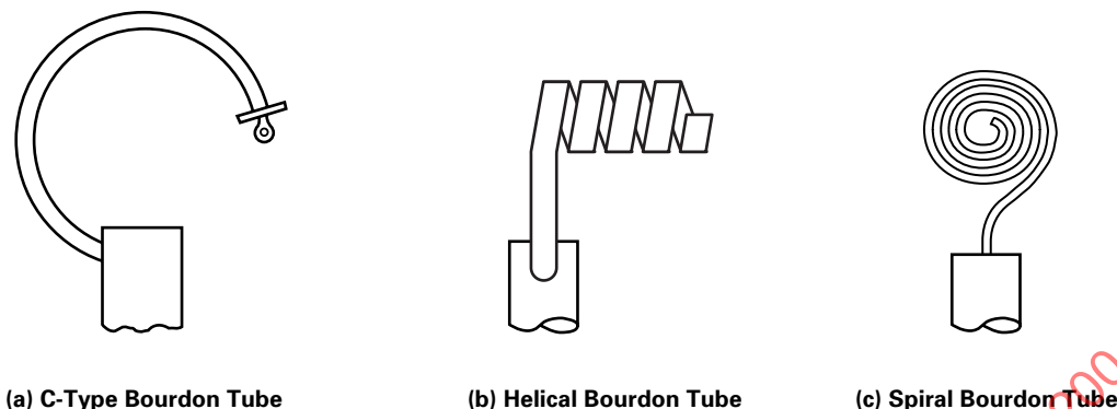
Fig. 2 Elastic Elements
