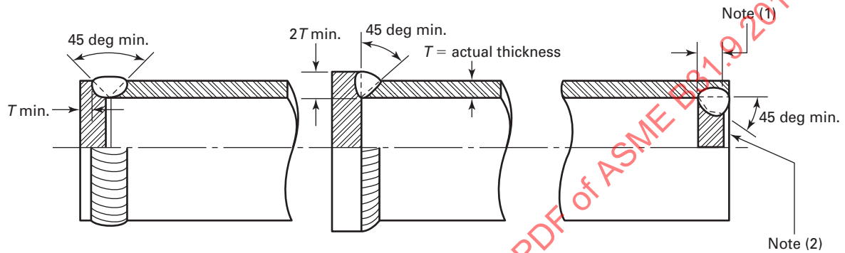
Fig. 927.4.5-1 Acceptable Welds for Flat Heads
