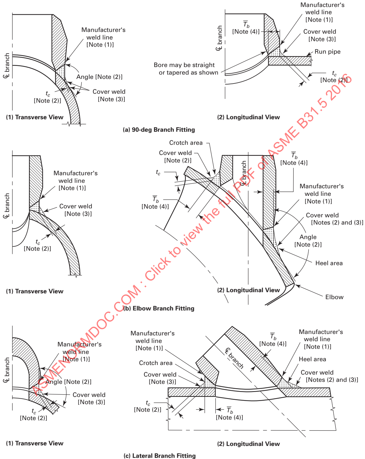
(16) Fig. 527.3.5-5 Some Acceptable Details for Integrally Reinforced Outlet Fittings
