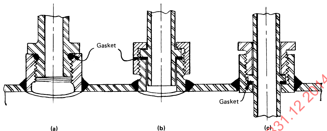
Fig. IP-9.14-1 Typical Threaded Joints Using Straight Threads
