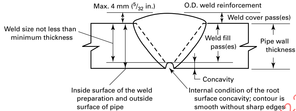
Fig. GR-3.4.6-1 Geometry of Weld Deposit Single Vee Groove Butt, Open Root With Concavity
