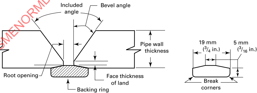
Fig. GR-3.4.3-7 Geometry of Weld Joint Detail Single Vee Groove Butt, Continuous Tapered Backing Ring
