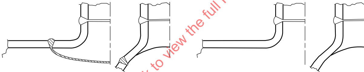
Fig. GR-3.4.9-4 Acceptable Details for Branch Attachment Suitable for 100% Radiography
