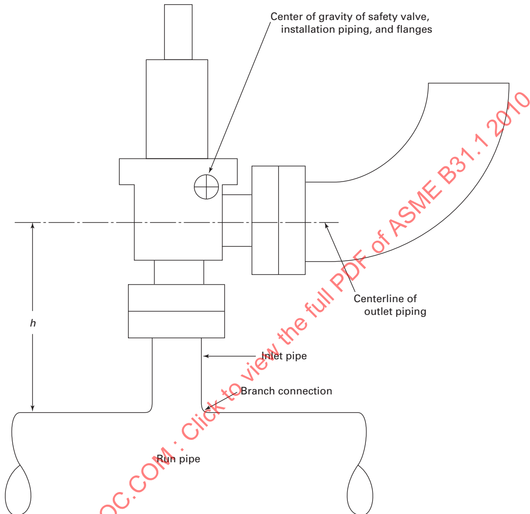
Fig. II-3-1 Safety Valve Installation (Open Discharge System)
