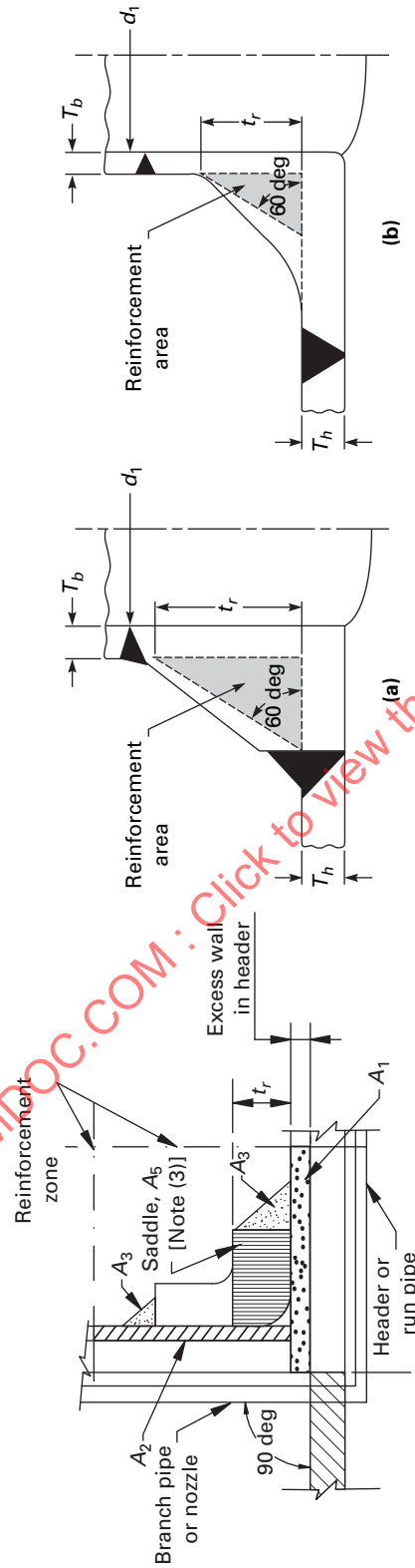
Fig. 104.3.1(D) Reinforcement of Branch Connections (Cont'd)
