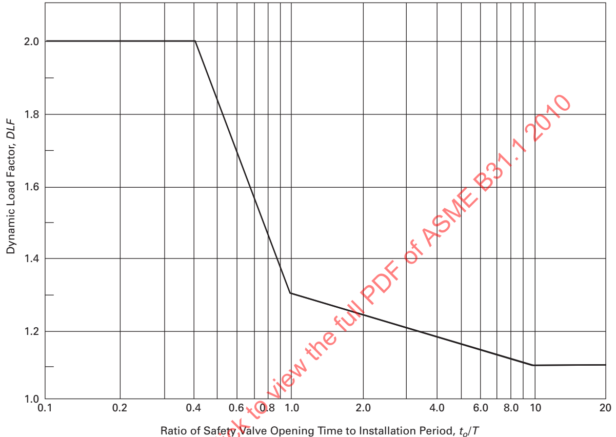
Fig. II-3-2 Dynamic Load Factors for Open Discharge System
