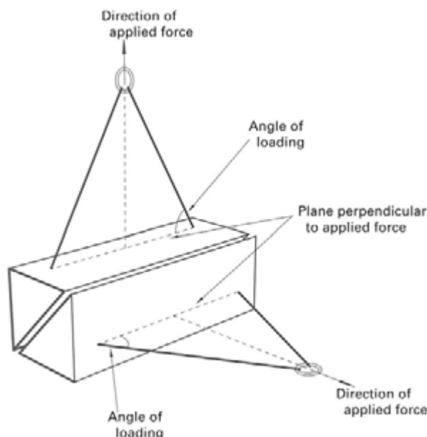
Fig. 9-1.5-1 Angle of Loading
