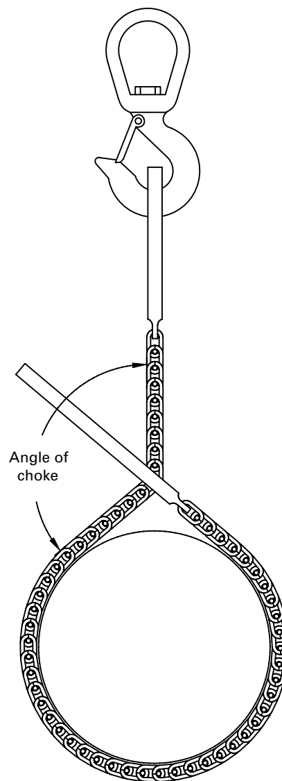
Fig. 9-3.10.1-1 Angle of Choke: Metal Mesh Slings
