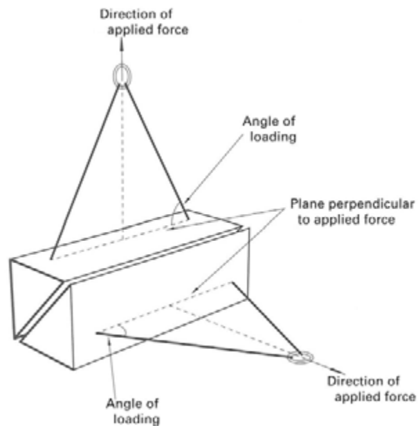
Fig. 9-5.5-1 Angle of Loading
