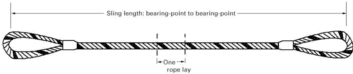
Fig. 9-2.0-1 Wire Rope Sling
