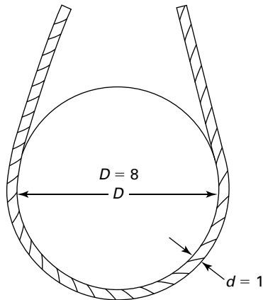
Fig. 9-4.10.1-1 D/d Ratio: Synthetic Rope Slings
