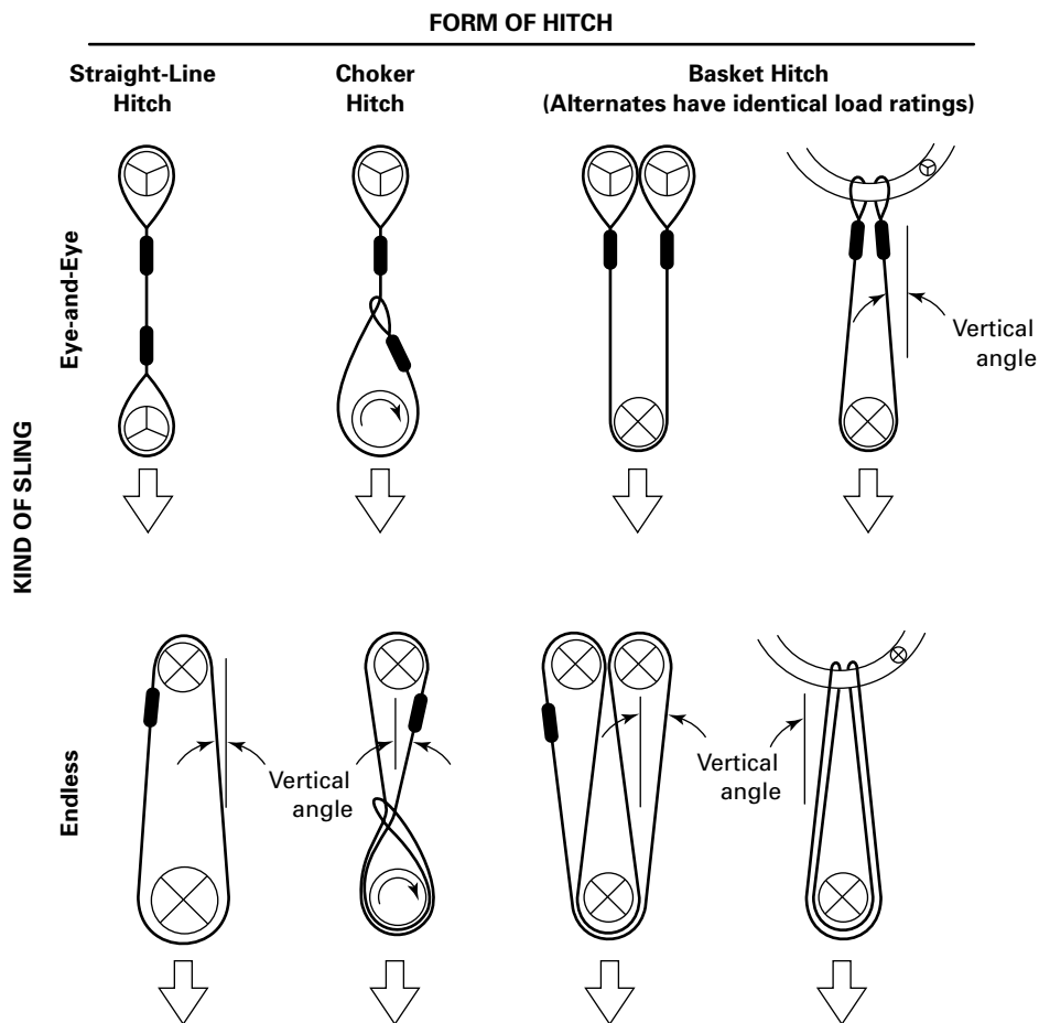
Fig. 9-4.5-1 Hitch Types for Synthetic Rope Slings
