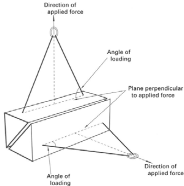
Fig. 9-6.5-1 Angle of Loading
