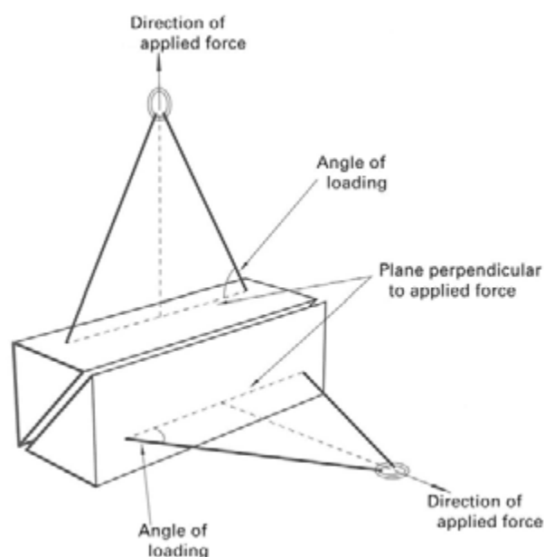
Fig. 9-2.5-1 Angle of Loading
