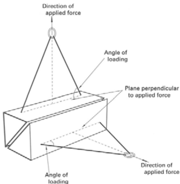
Fig. 9-3.5-1 Angle of Loading
