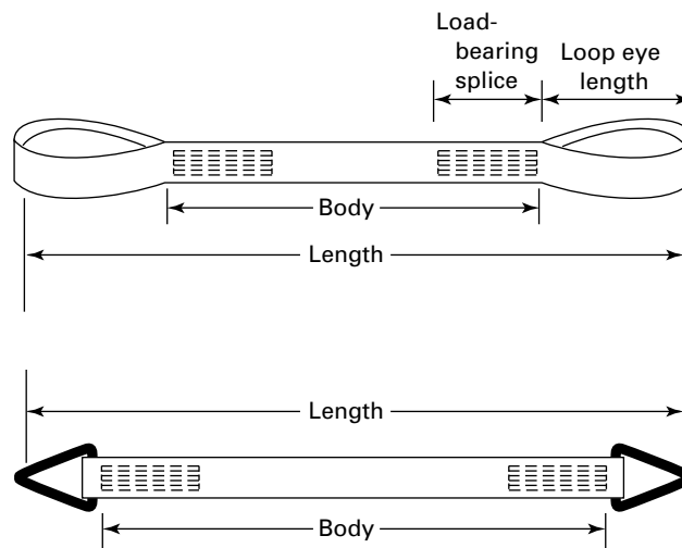
Fig. 9-5.0-2 Synthetic Webbing Sling Nomenclature
