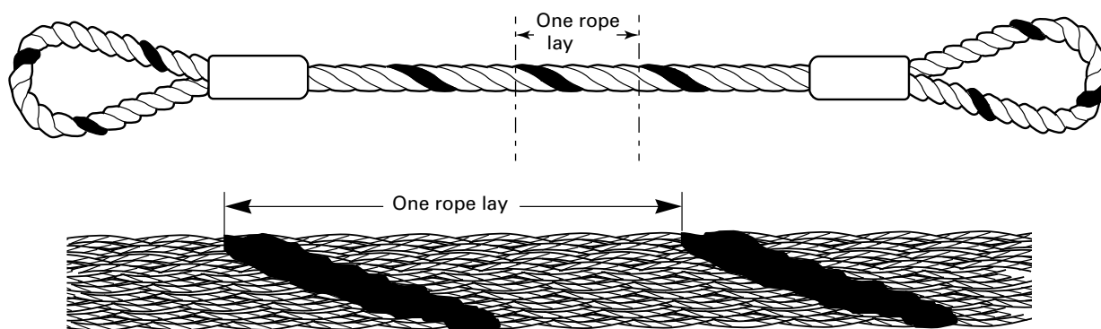
Fig. 9-2.9.5-1 Cable-Laid Wire Rope Sling
