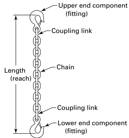
(b) Single-Leg Sling Components
