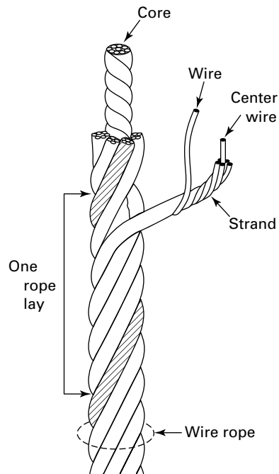
Fig. 9-2.0-2 Wire Rope
