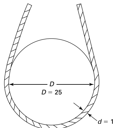
Fig. 9-2.10.1-1 D/d Ratio: Wire Rope Slings
