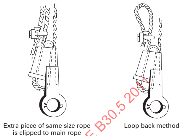
Fig. 5-1.7.3-1 Dead Ending Rope in a Socket
