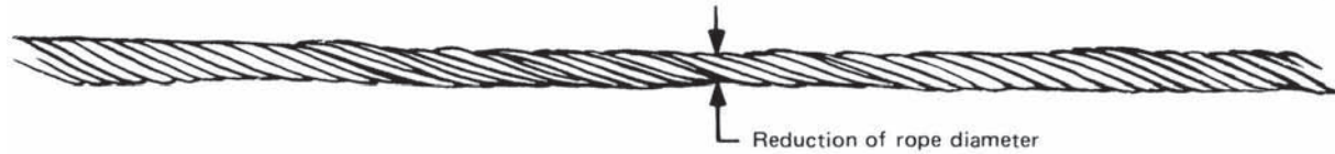
Fig. 5-2.4.2-1 Core Failure in 19 \times 7 Rotation-Resistant Rope (Note the lengthening of lay and reduction of diameter)
