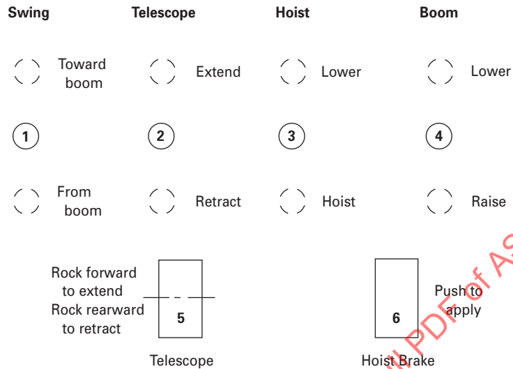
Fig. 5-1.6.1-1 Telescopic Boom Crane Control Diagram (Suggested Mobile Telescopic Boom Crane Basic Operating Control Arrangement for New Cranes)
