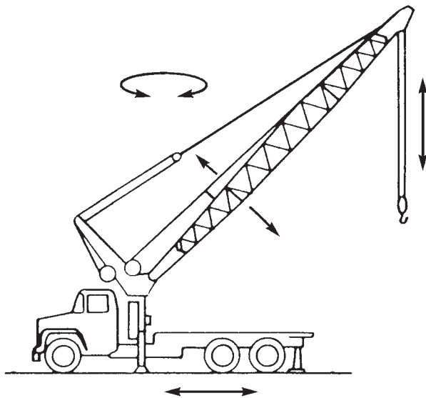
Fig. 5-0.2.1-2 Commercial Truck-Mounted Crane — Nontelescoping Boom
