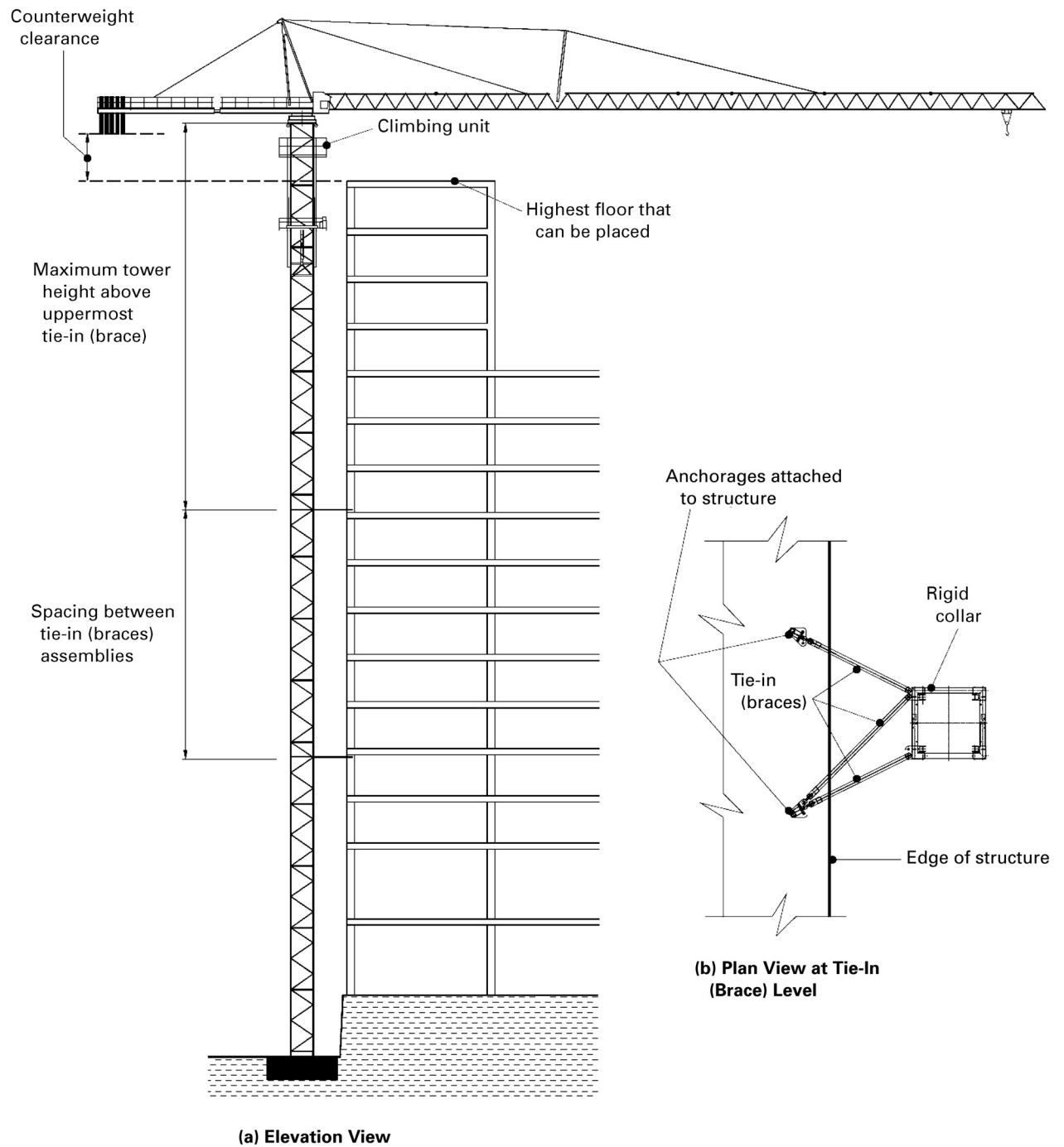
Fig. 3-0.2.1.3-1 Braced Crane
