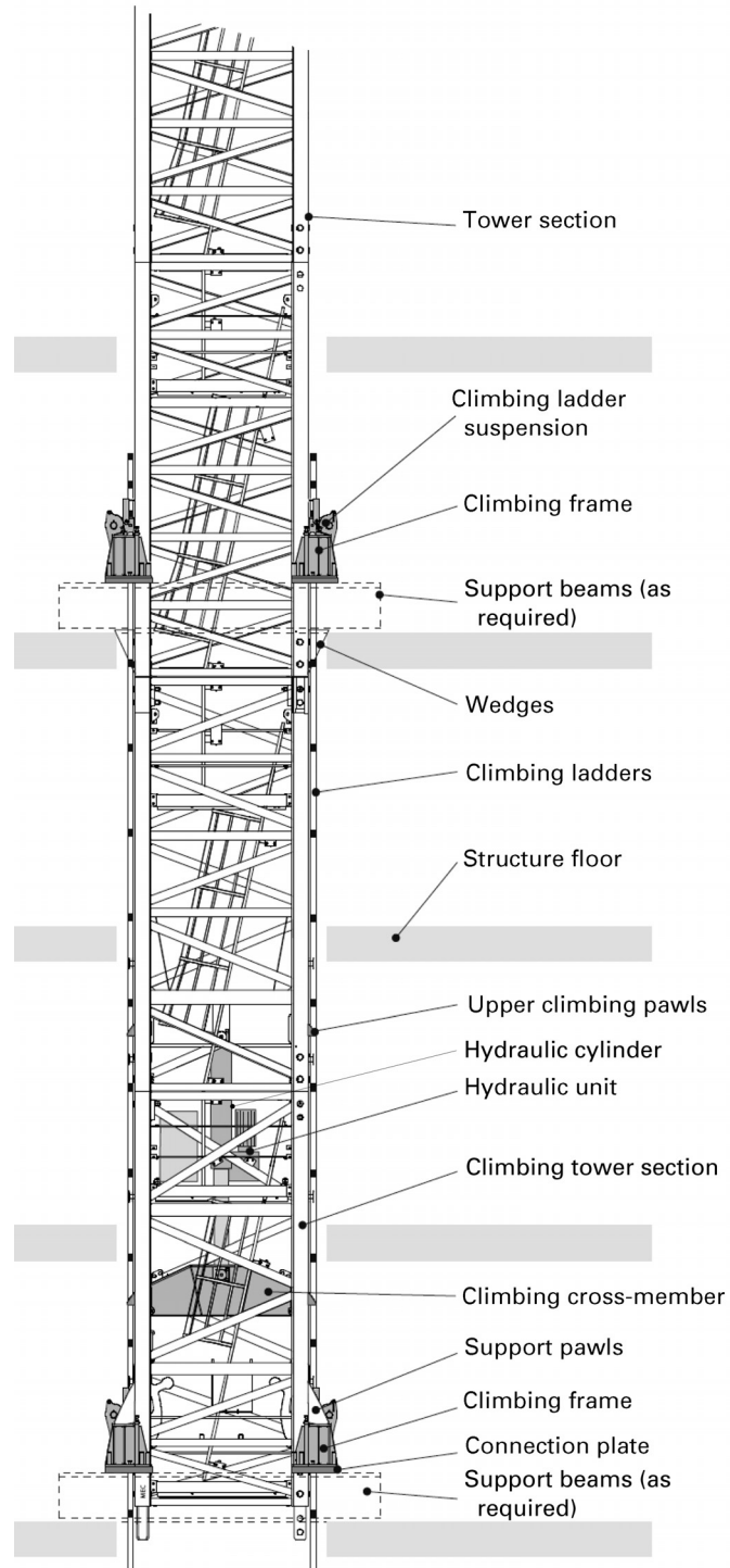
Fig. 3-0.2.1.3-2 Internal Climbing Crane
