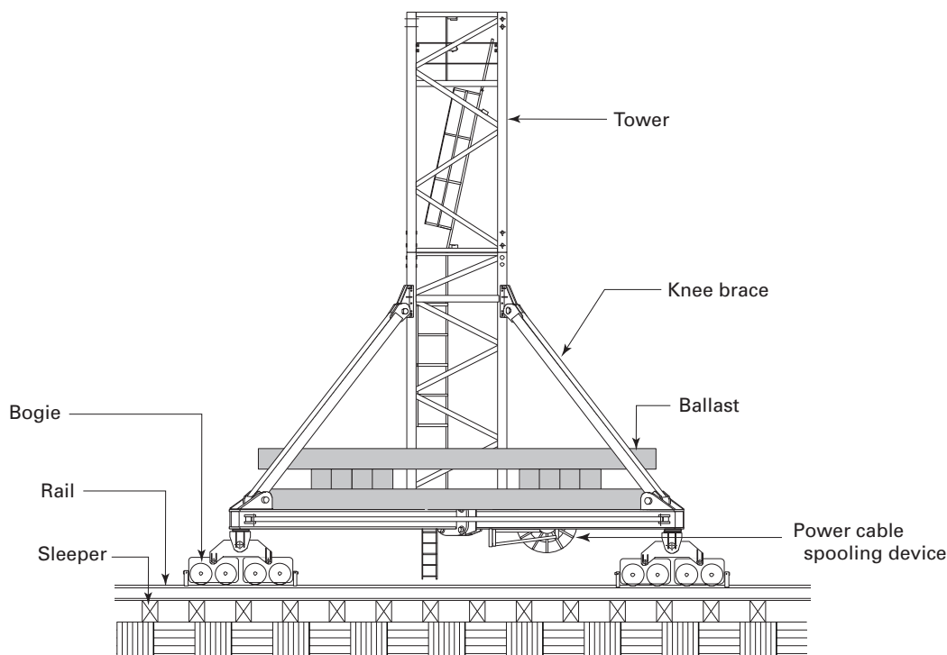
Fig. 3-0.2.1.4-1 Travel Base for Freestanding Crane
