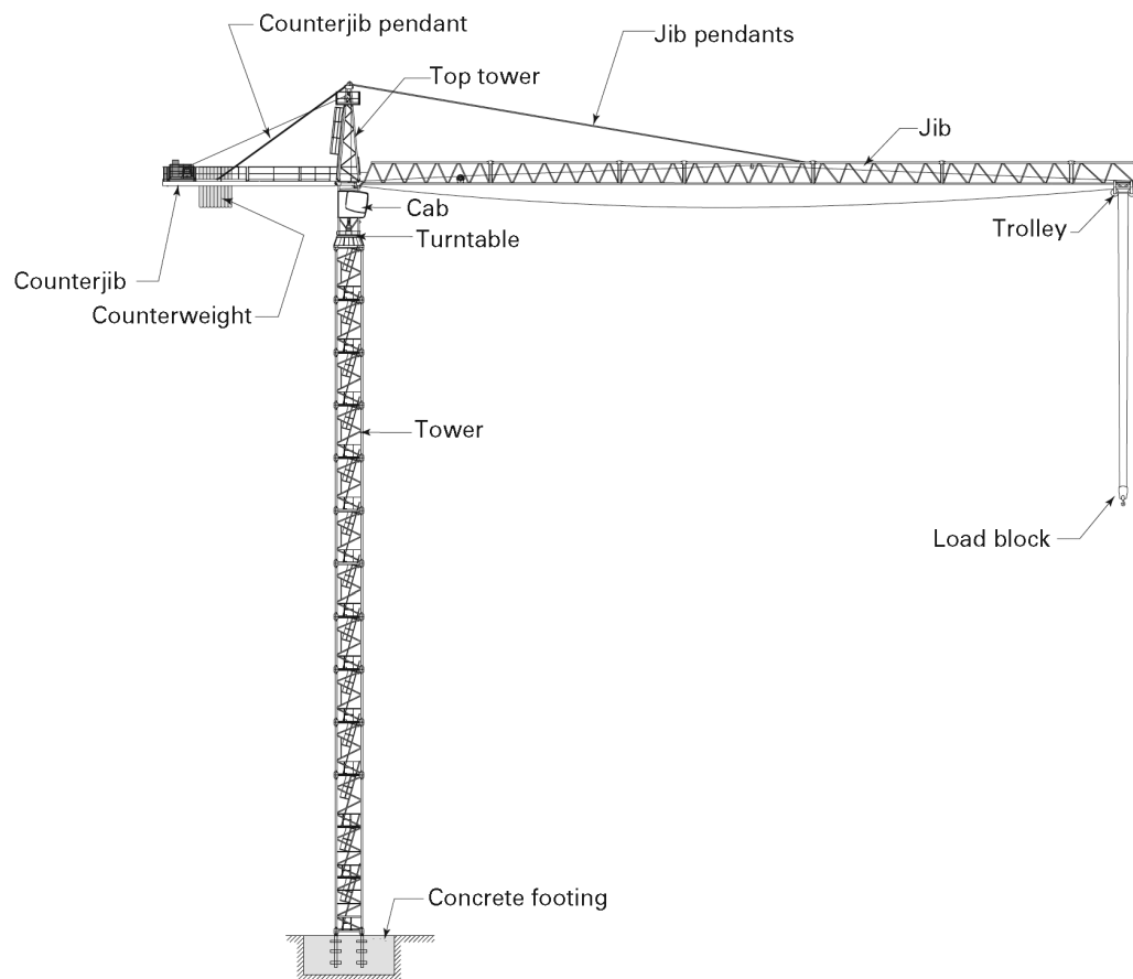
Fig. 3-0.2.1.2-1 Hammerhead Tower Crane — Fixed-Base, Freestanding Crane
