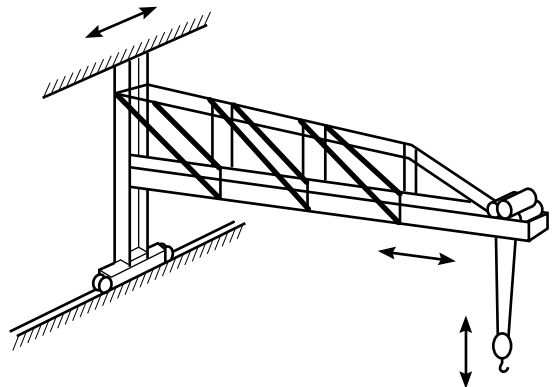
Figure 2-0.2-5 Wall Crane
