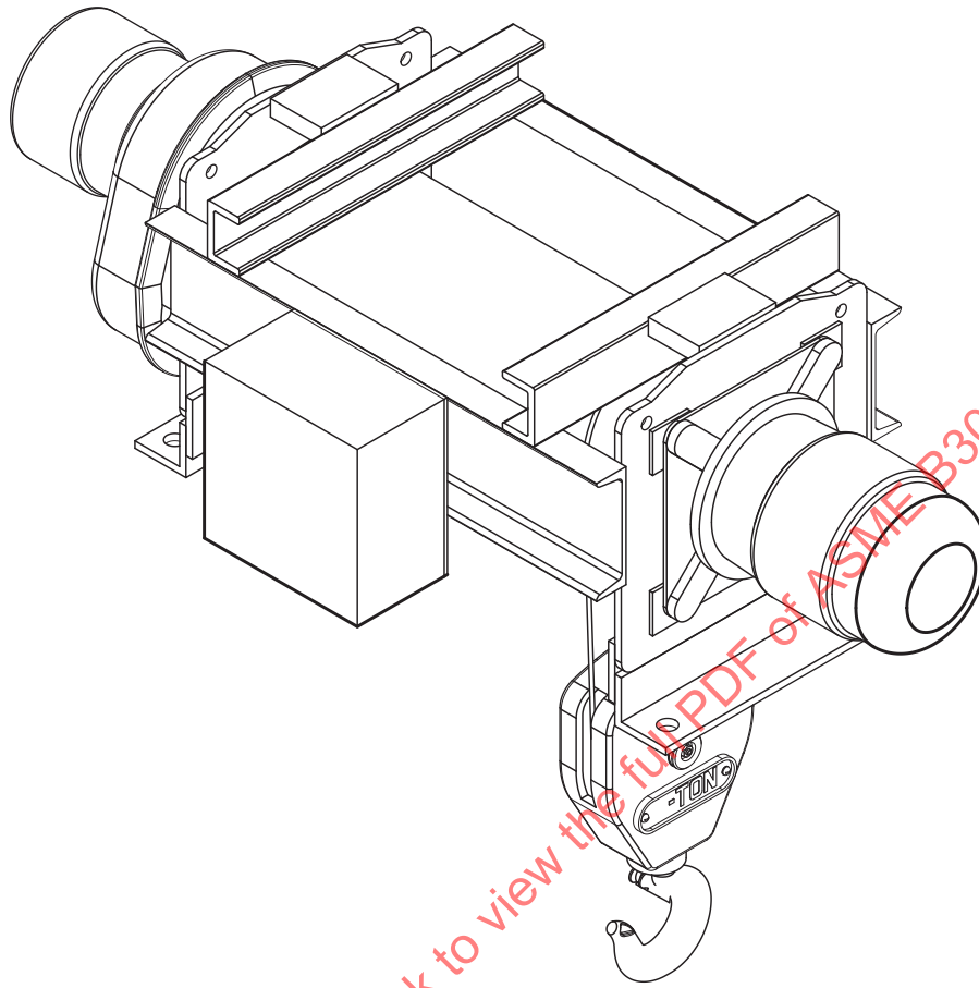
Fig. 16-0.1-6 Stationary Hoist
