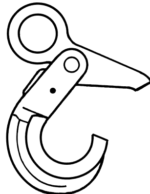
Fig. 10-1.1-6 Self-Locking Eye Hook (Open)
