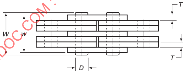
3 × 4 Lacing
