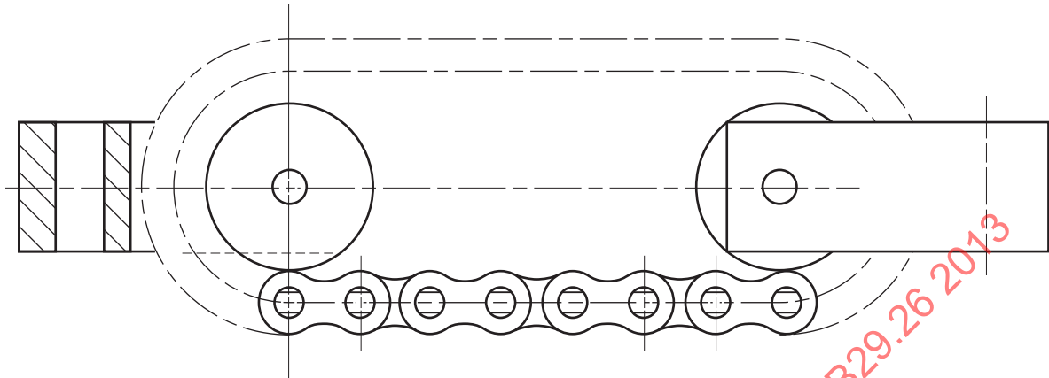
Fig. 5 Typical Fatigue Test Fixtures for Endless Chain Tested on Sprockets or Sheaves
