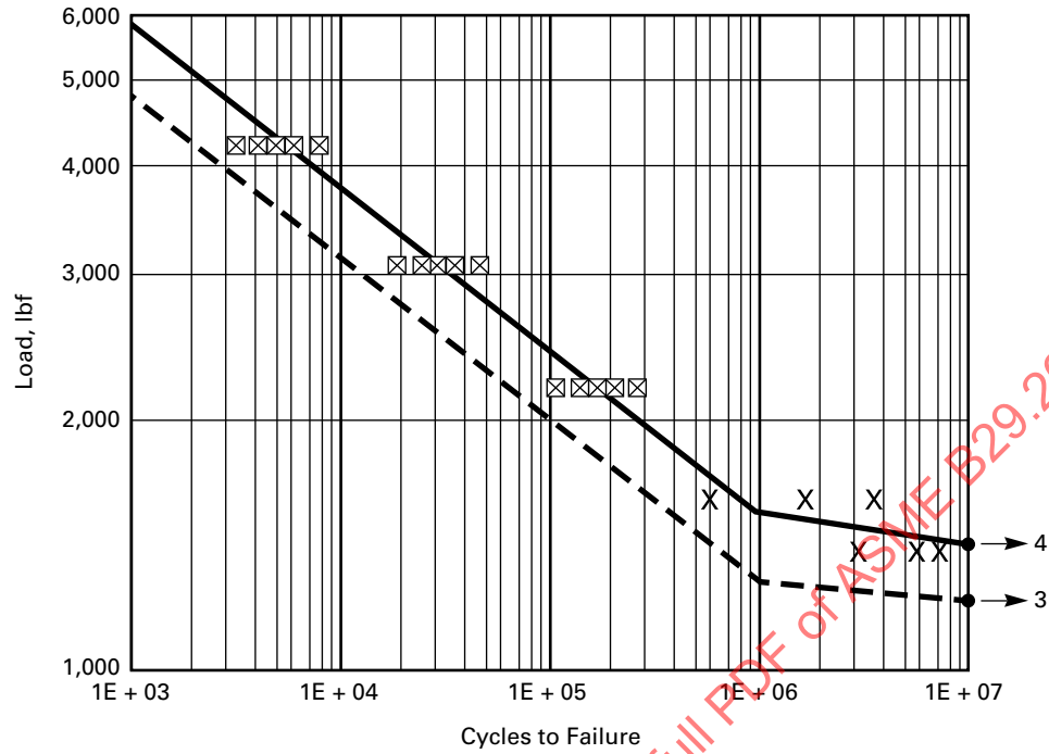
Fig. 8 Typical Fatigue Test Data Plot
