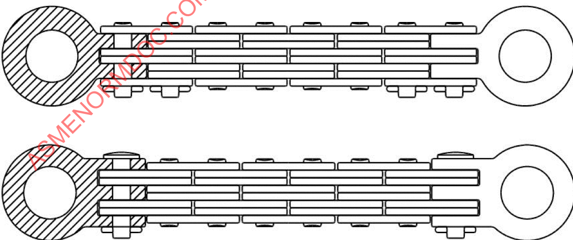
Fig. 4 Typical Leaf Chain Fatigue Test Specimens and Fixtures
