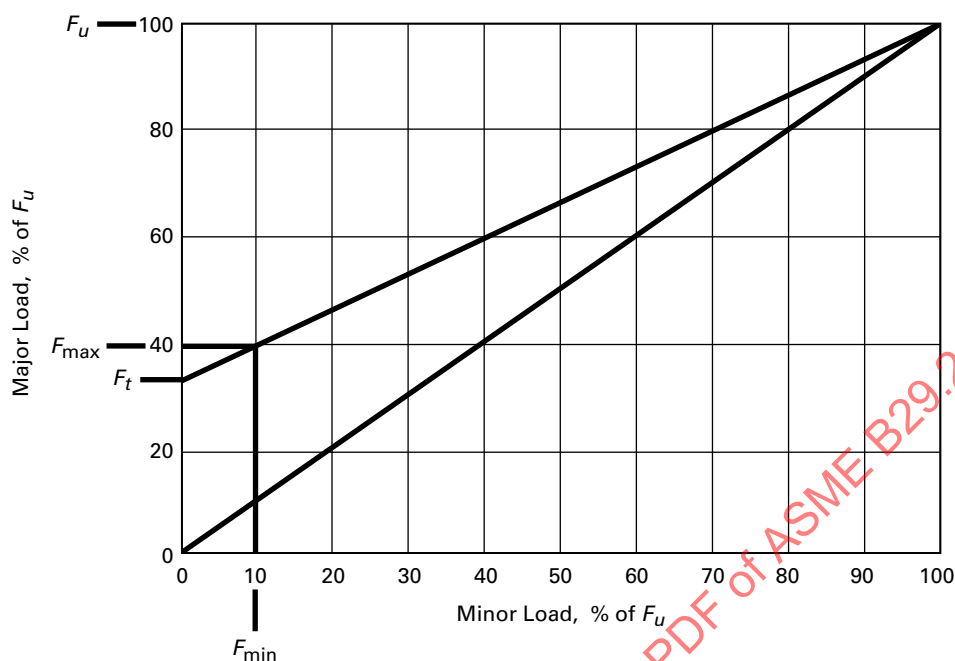
Fig. 6 Johnson-Goodman Diagram
