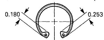
Alternate Design for Size -118 (Manufacturer's Option)
