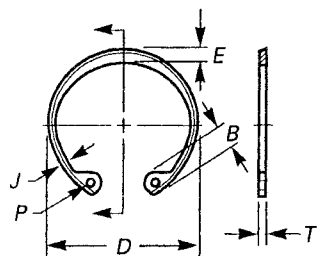
Free Diameter and Ring Measurements
