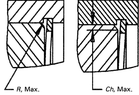
Maximum Corner Radius &amp; Chamfer
