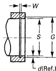
Housing Diameter and Groove Dimensions
