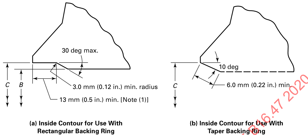
Figure 2 Welding Ends (Welding Neck Flanges With Backing Rings)
