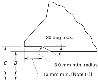
(a) Inside Contour for Use With Rectangular Backing Ring
