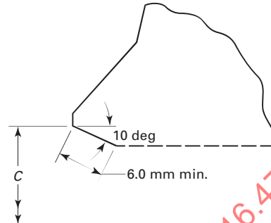
(b) Inside Contour for Use With Taper Backing Ring
