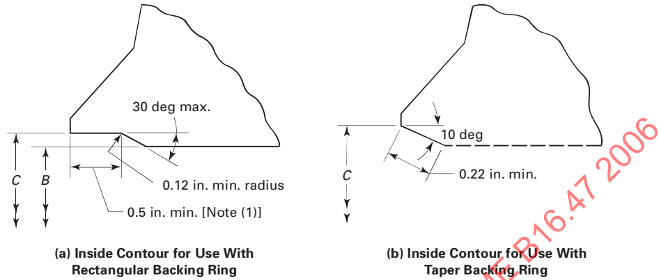
Fig. I-2 Welding Ends (Welding Neck Flanges With Backing Rings)
