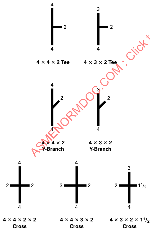
Figure 4.2-1 Identification of Reducing Fittings
