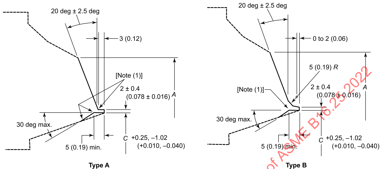
Figure 3.2-2 Weld Bevel Details for GTAW Root Pass [Wall Thickness Over 10 mm to 25 mm (0.38 in. to 1.0 in.), Inclusive]
