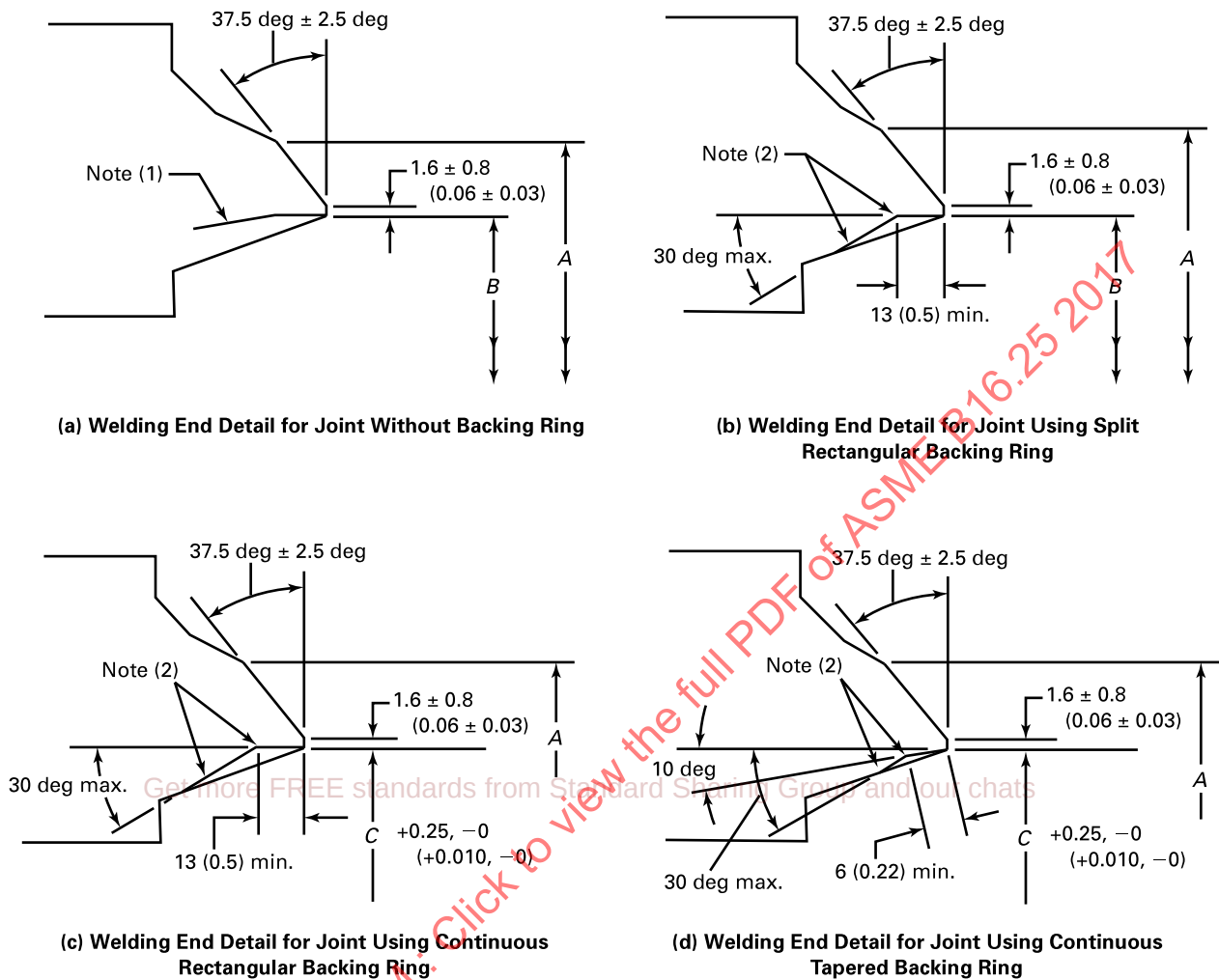
Figure 2 Bevels for Wall Thickness Over 3 mm (0.12 in.) to 22 mm (0.88 in.), Inclusive
