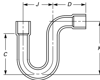
C x C Suction Line P-Traps
