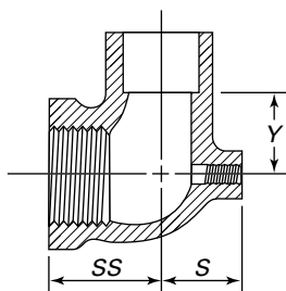
Baseboard Tee F × F × C
