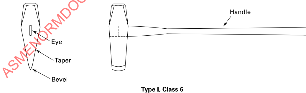
Figure 5.4.1-2 Category 48 Type I Handle-Held Chisels
