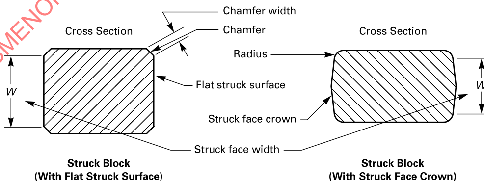
Figure 5.8-3 Struck Block Cross Section
