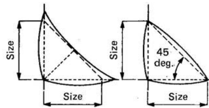
(a) Desirable Fillet Weld Profiles
