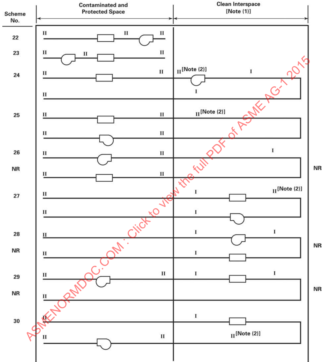
FIG. SA-B-1410-3 RECIRCULATING AIR CLEANING SYSTEM CONFIGURATIONS
