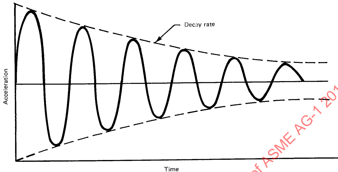
FIG. AA-4355.4 SINE AMPLITUDE DECAY RATE
