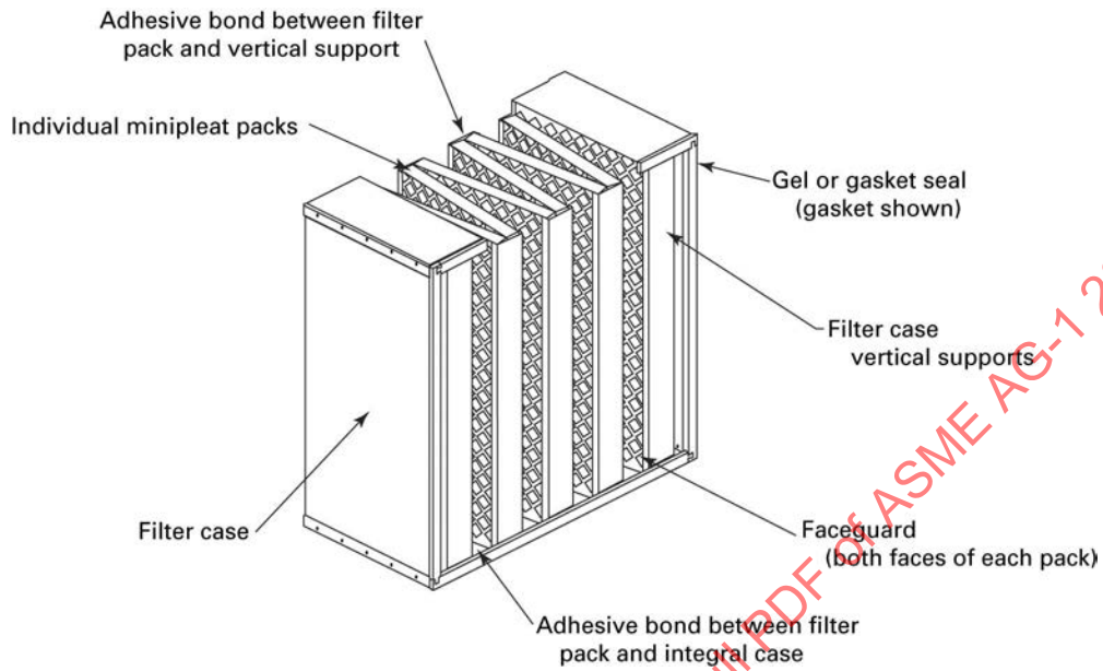
FIG. FC-4110-3 TYPE B MINIPLAT FILTER
