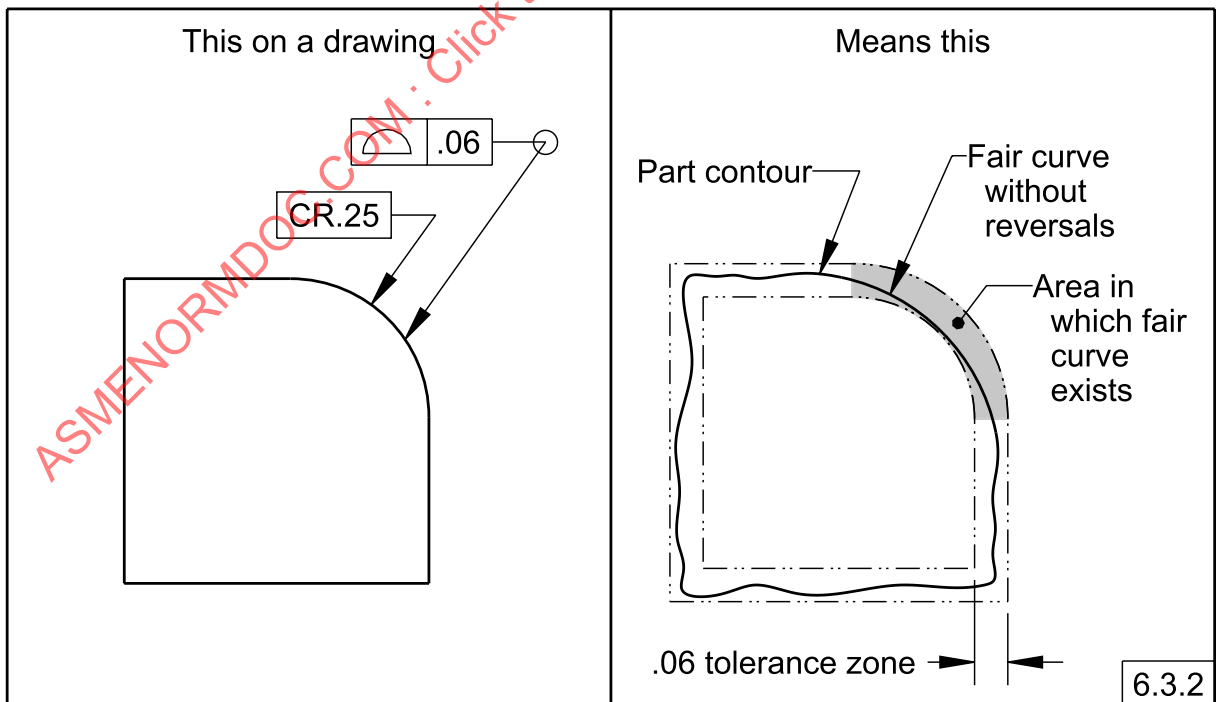
Figure 6-7 Controlled Radius
