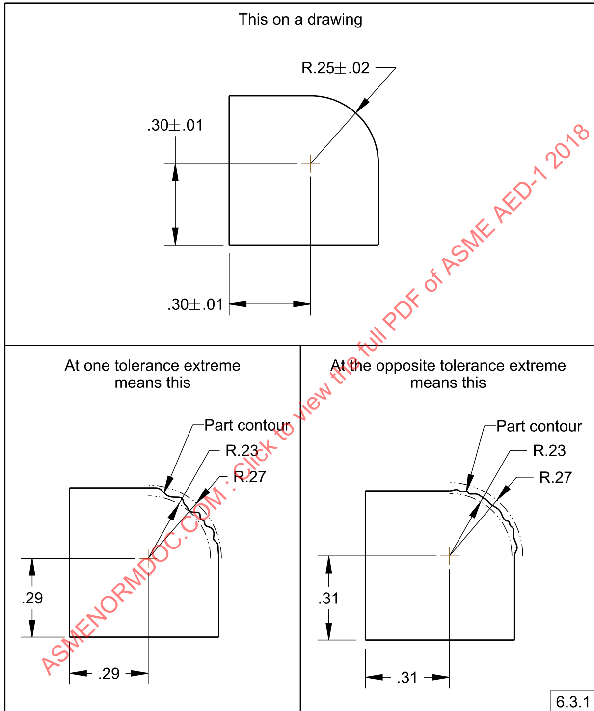
Figure 6-5 Center-Located Radius
