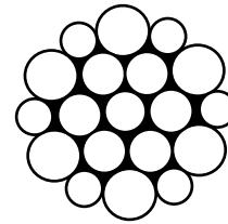
Figure 1.3.1.3.4-3 Filler Construction (e.g., 25F, 12-6F-6-1)
