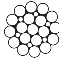
Fig. 1.3.1.3.4-3 Filler Construction (e.g., 25F, 12-6F-6-1)
