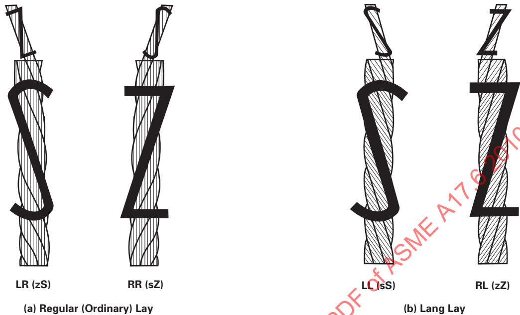
Fig. 1.3.2.4.2-1 Regular (Ordinary) Lay and Lang Lay
