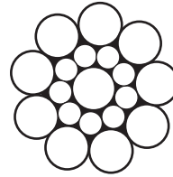
Fig. 1.3.1.3.4-1 Seale Construction (e.g., 19S, 9-9-1)
