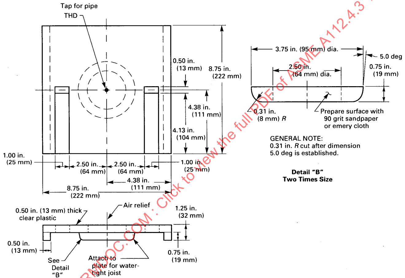
FIG. 3 TEST FIXTURE 2
